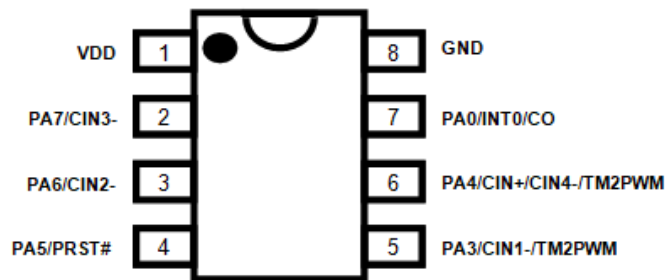
PMS150C-S08 (SOP8-150mil)
